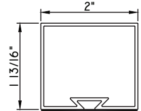
2"X1 13/16" M23199
